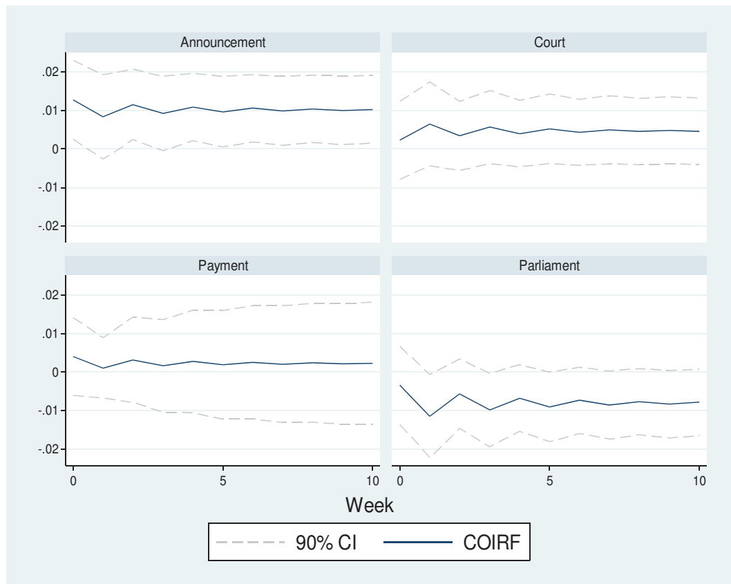
Figure 2B: Cumulative Orthogonalized Impulse Response
