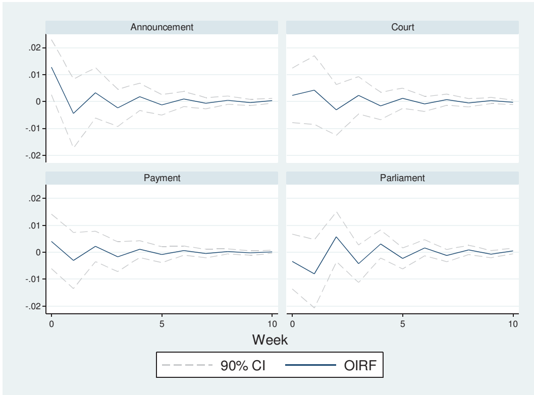
Figure 2A: Orthogonalized Impulse Response
