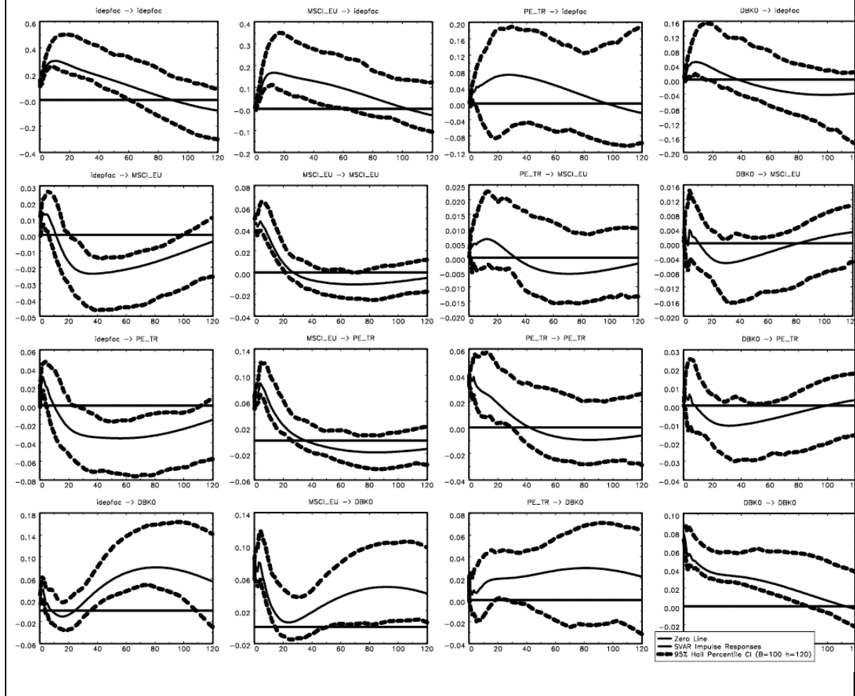
Figure 4b SVAR Impulse Responses, k = 4 Sample 2005.1-2023.9:
