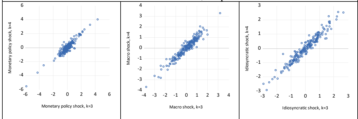
Figure 4c Correlations of structural residuals, sample 2005.1-2022.6
