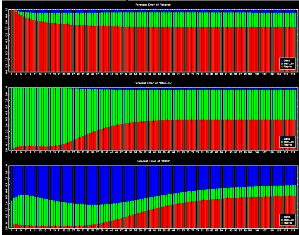
Figure 3b FEVDs, k = 3 Sample 2005.1-2023.9:
