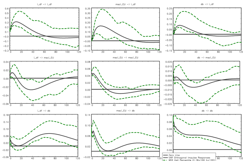
Figure 3. SVAR Impulse Responses, k=3 , Sample 2005.1-2023.9.
